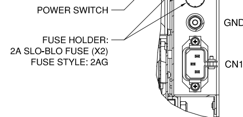
SECTION E-E
