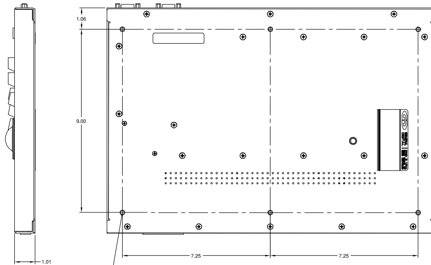
#10-32 BLIND PEM FASTENERS FOR CUSTOMER MOUNTING (x6)
