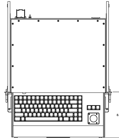
Top View: 2U Rack Mount Keyboard Extended
