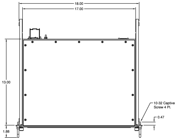
Top View: 2U Rack Mount Keyboard Stowed
