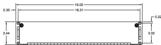
Front View: 2U Rack Mount Keyboard Stowed
