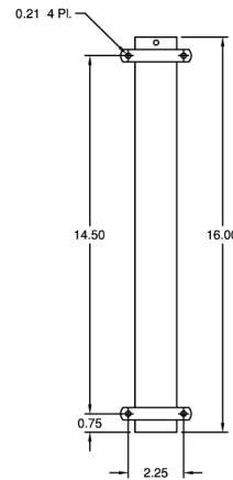
Stationary Slide Section
