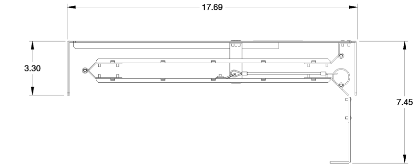
STOWED POSITION
