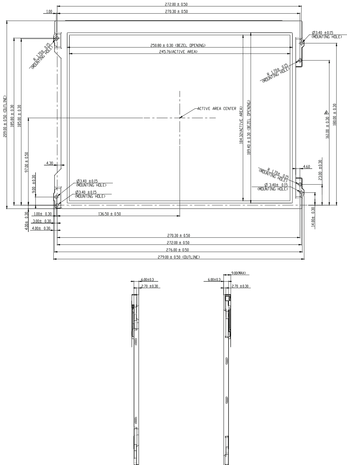
Figure 4: Display dimensions (unit of measure: mm; tolerance is ±0.50 mm unless otherwise indicated)
